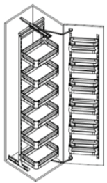
CODE 45006 Pull Out Pantry Unit 450mm Cabinet W414xD500xH1850-2150mm
