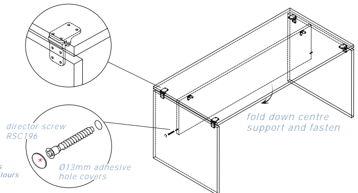
WEDGE FITTING | ITEM 1280
