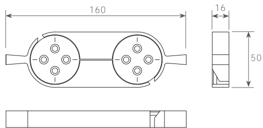
FOLD AWAY HINGE | ITEM 590
